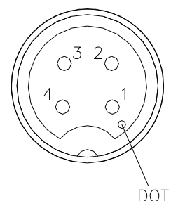
EN3L4F PINOUT FRONT VIEW
